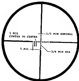
Figure 2-23. Reticle.
